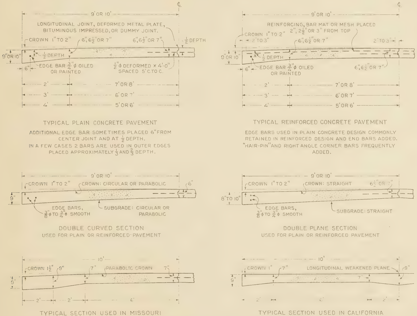
FIGURE 1.—TYPICAL CROSS-SECTION DESIGNS
